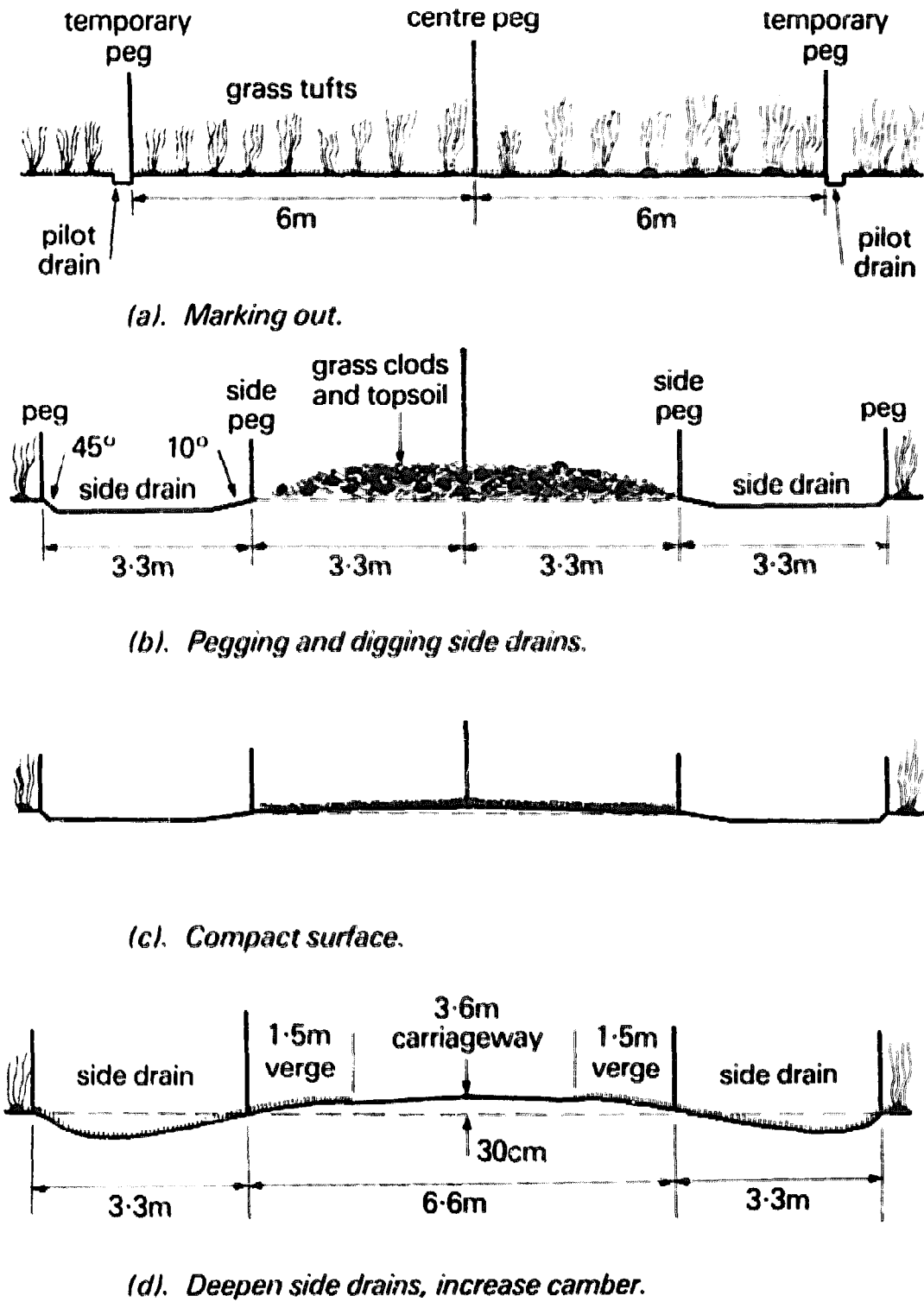
Figure 40. Construction of embanked road in wet area.
